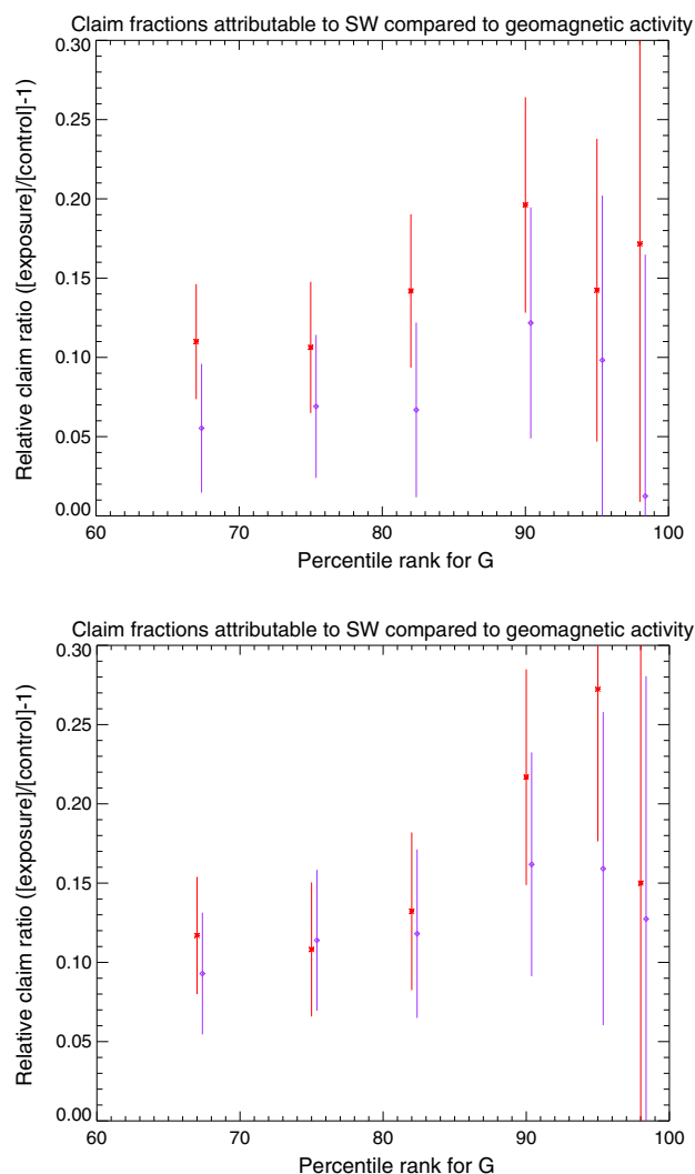
Figure 11. Relative excess claim frequencies (n_i - n_c)/n_i on geomagnetically active dates relative to those on control dates for geomagnetic latitudes below 49.5^\circ\text{N} (asterisks, red) compared to those for higher latitudes (diamonds, purple; offset slightly to the right) for the percentiles tested (98, 95, 90, 82, 75, and 67). (top) The results for the full sample (A) and (bottom) for sample B from which apparently nonspace weather-related events were removed (see section 2.1).
