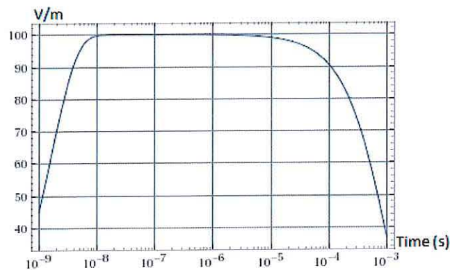
Figure 2. Recommended E2 benchmark waveform.
