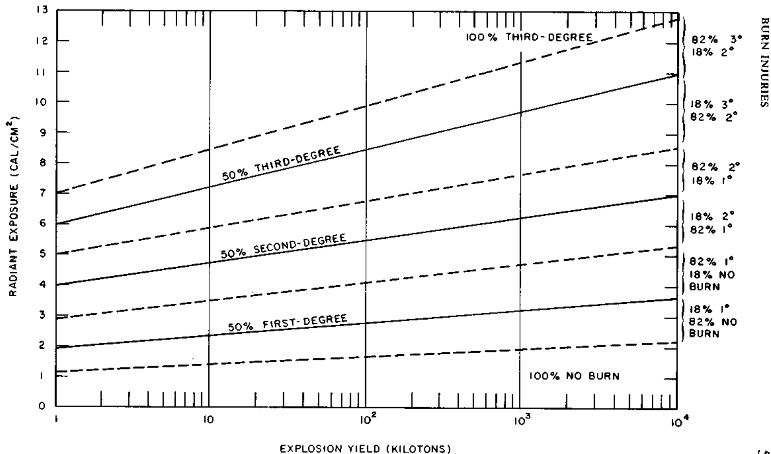
Figure 12.65. Skin burn probabilities for an average unshielded population taking no evasive action as a function of explosion yield and radiant exposure.
