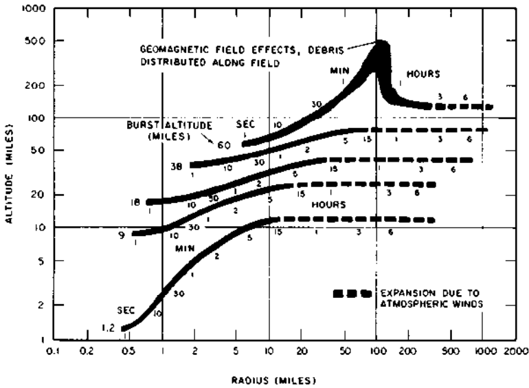
Figure 10.158c. Fireball/debris altitude and horizontal radius for 1-megaton explosions at various altitudes.
