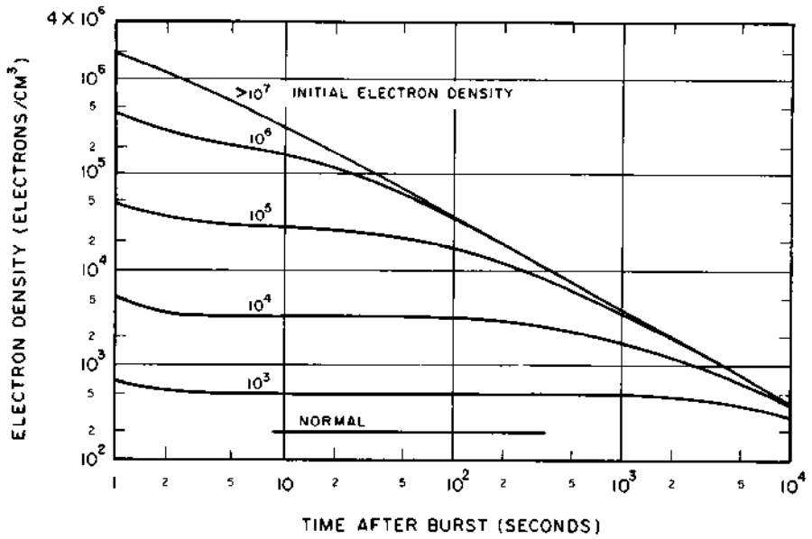
Figure 10.151. Decay of ionization from prompt radiation at 40 miles altitude in the daytime.
