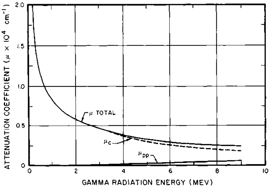
Figure 8.97b. Linear attenuation coefficient of air as function of gamma-ray energy.
