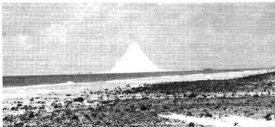
Figure 2.84a. Spray dome observed 5.3 seconds after explosion in deep water.
