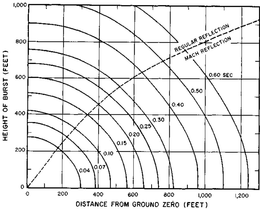
Figure 3.77a. Arrival times on the ground of blast wave for 1-kiloton burst (early times).
