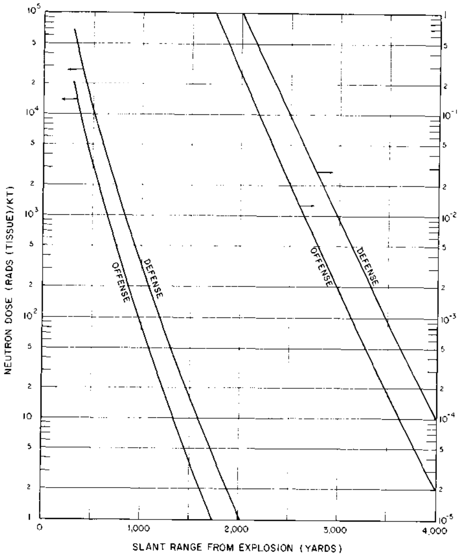
Figure 8.123a. Initial neutron dose per kiloton total yield as a function of slant range from fission weapon air bursts, based on 0.9 normal sea-level air density.
