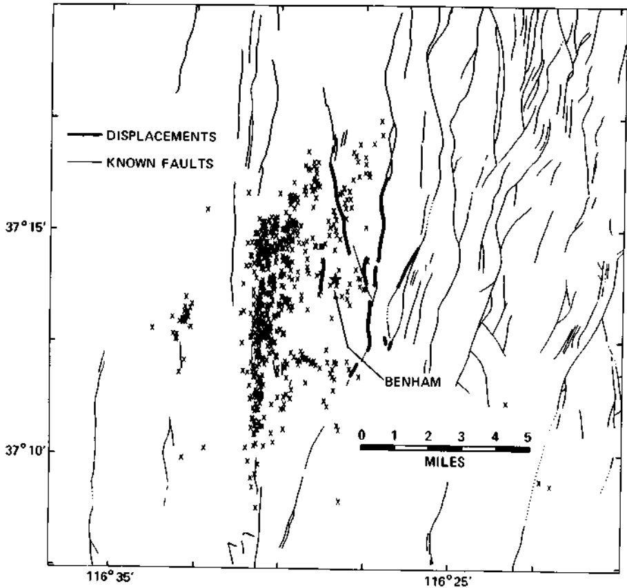
Figure 6.21. Locations of 640 aftershocks and fault displacements from the BENHAM 1.1-megaton test.
