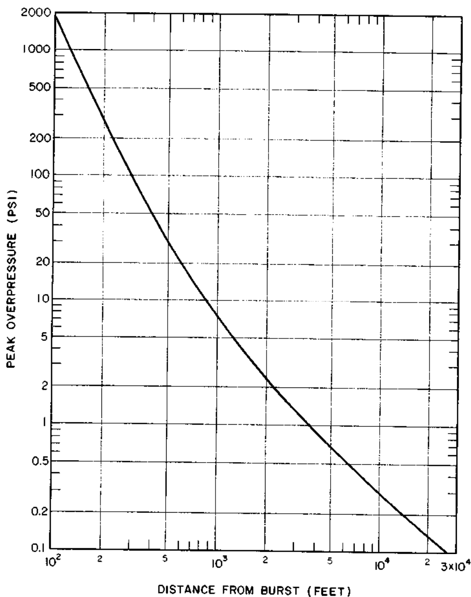
Figure 3.72. Peak overpressure from a 1-kiloton free air burst for sea-level ambient conditions.
