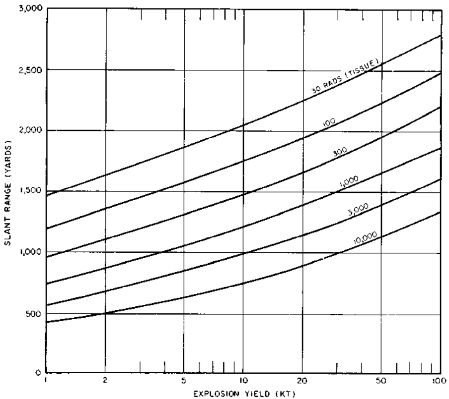
Figure 8.33a. Slant ranges for specified gamma-ray doses for targets near the ground as a function of energy yield of air-burst fission weapons, based on 0.9 sea-level air density. (Reliability factor from 0.5 to 2 for most fission weapons.)
