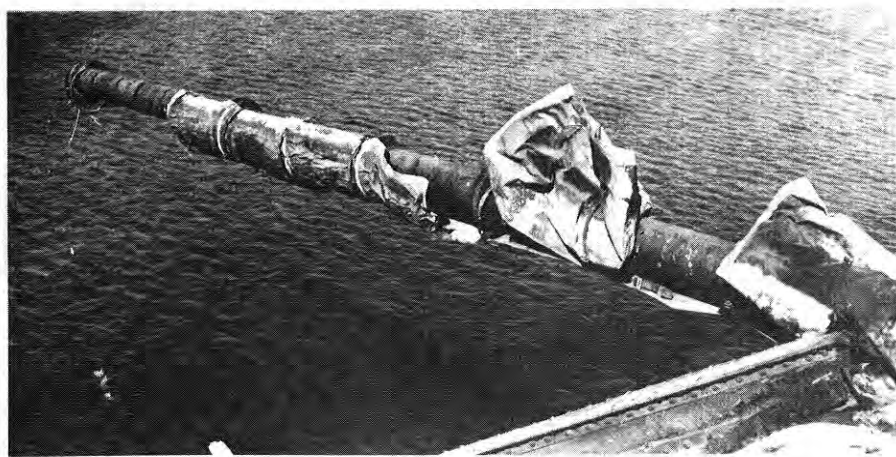
Figure 5.106b. Broken portion of 16-inch water main carried on bridge (0.23 mile from ground zero at Hiroshima).
