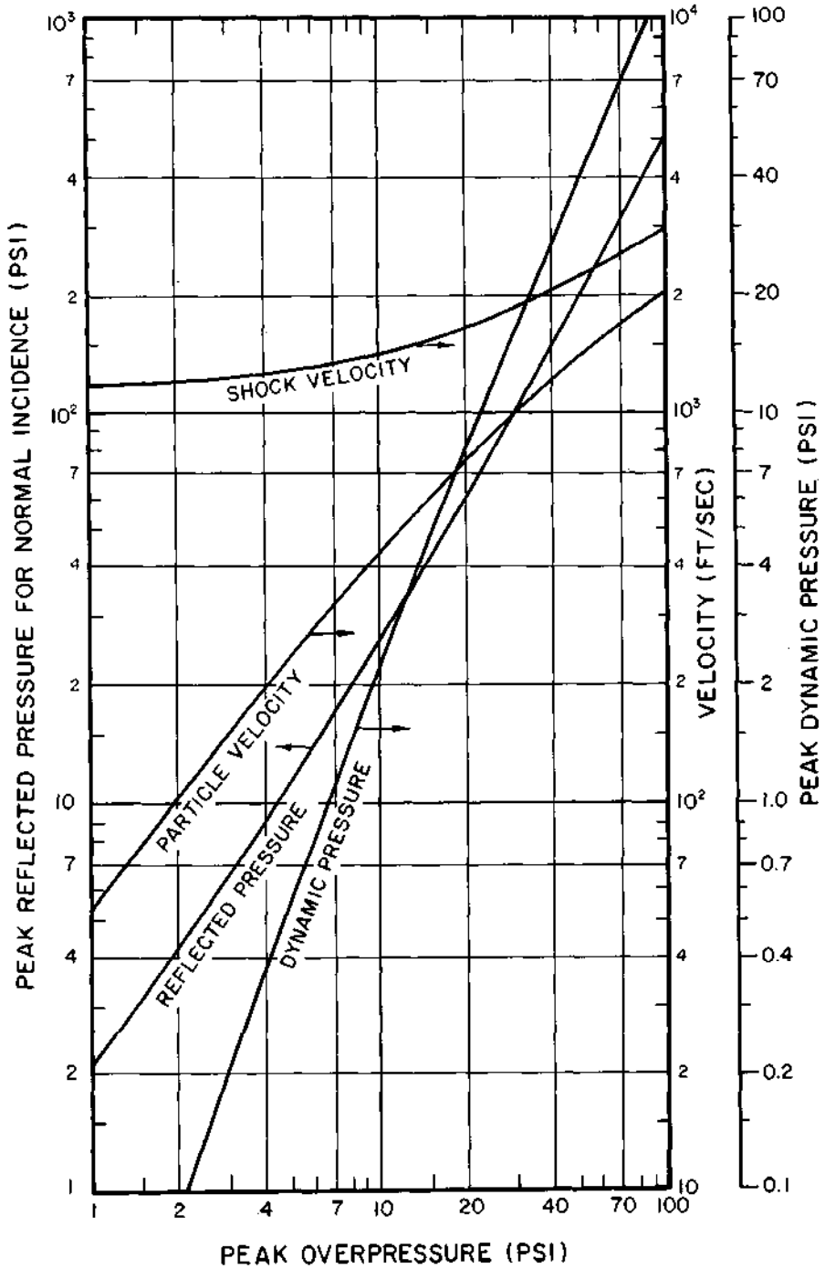
Figure 3.55. Relation of ideal blast wave characteristics at the shock front to peak overpressure.
