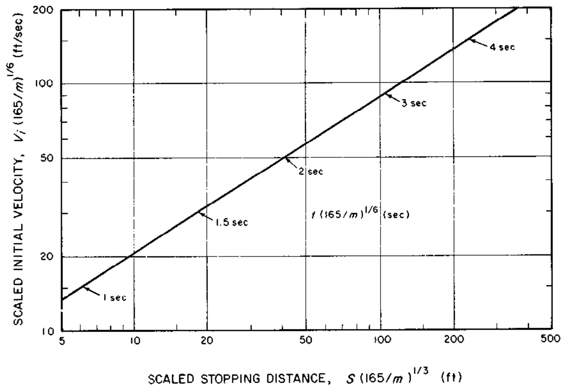
Figure 12.239. Initial velocity of animal ( V_i feet per second) scaled according to the mass (in pounds) versus the stopping distance for decelerative tumbling on a hard, flat surface. Scaled stopping times are indicated on the plot. (Estimated accuracy \pm 10 to 15 percent.)
