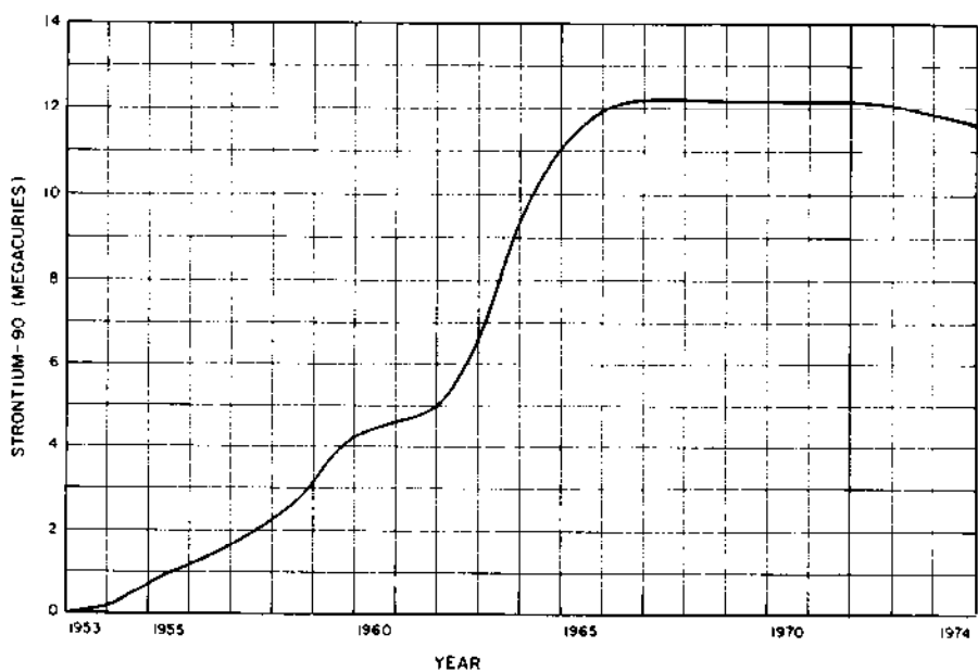
Figure 9.143b. Surface burden (or inventory) of strontium-90.
