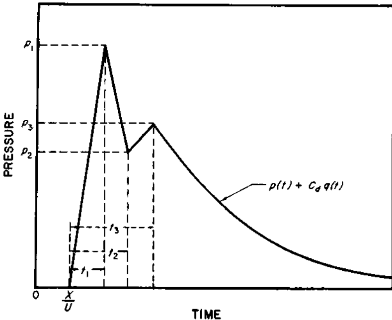
Figure 4.63. Typical pressure variation at a point on an arched structure subjected to a blast wave.
