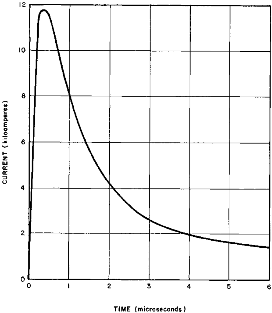
Figure 11.50. Typical form of the current pulse induced by the EMP from a high-altitude nuclear explosion in a long overhead power line. (The actual currents and times will depend to some extent on the conditions.)
