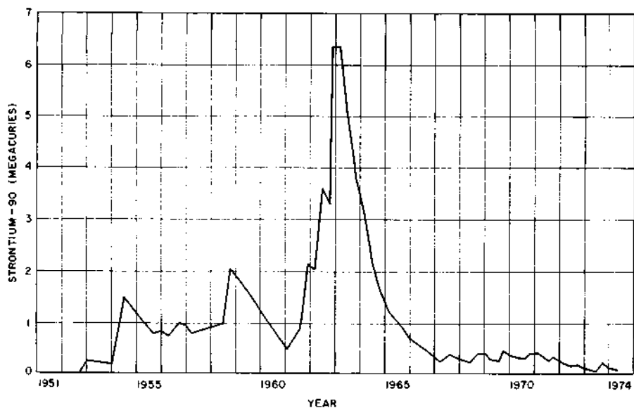
Figure 9.143a. Stratospheric burden (or inventory) of strontium-90.
