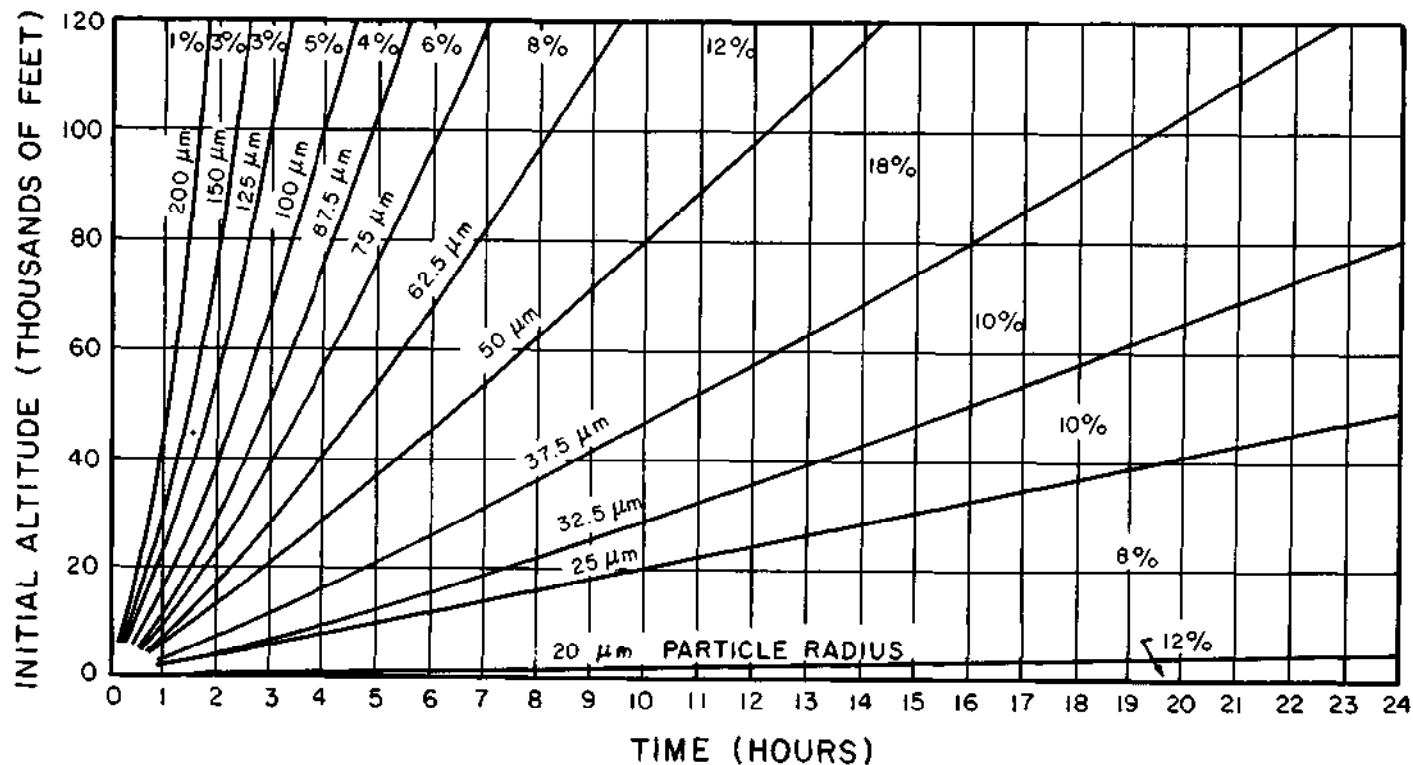
Figure 9.164. Times of fall of particles of different sizes from various altitudes and percentages of total activity carried.
