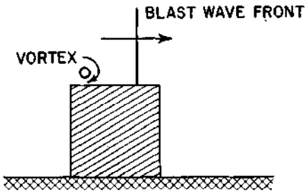
Figure 4.26. Blast wave moving over sides and top of cube.
