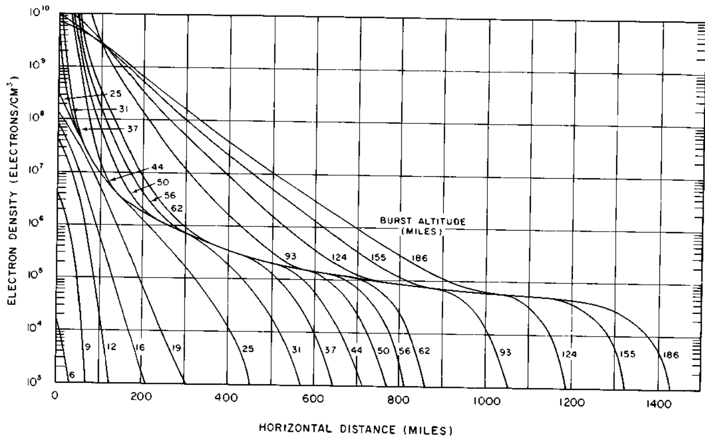
Figure 10.143. Initial electron density at 40-mile altitude produced by prompt radiation from a 1-megaton explosion, as a function of distance (miles), for various burst altitudes.
