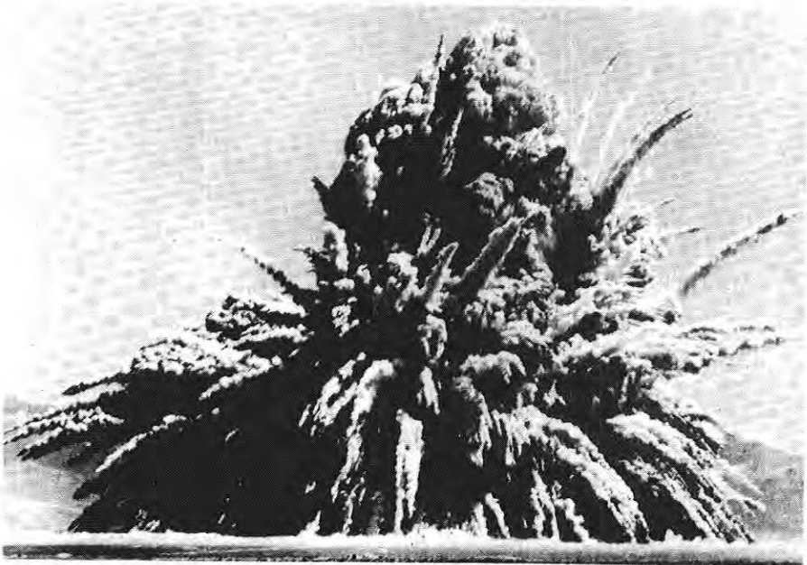
Figure 2.93. Shallow underground burst.
