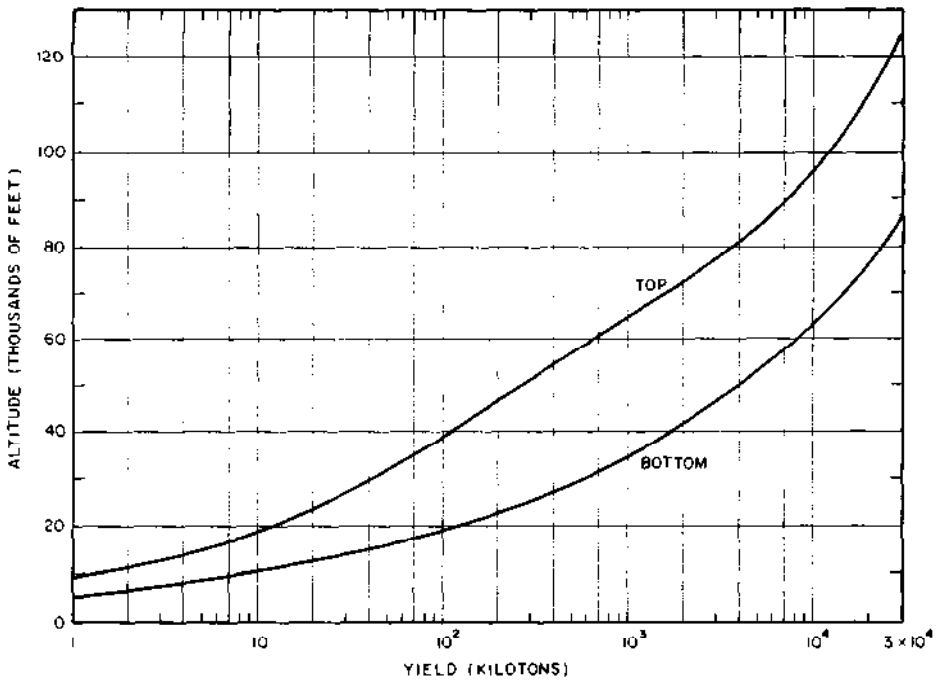
Figure 9.96. Altitudes of the stabilized cloud top and cloud bottom as a function of total energy yield for surface or low air bursts.
