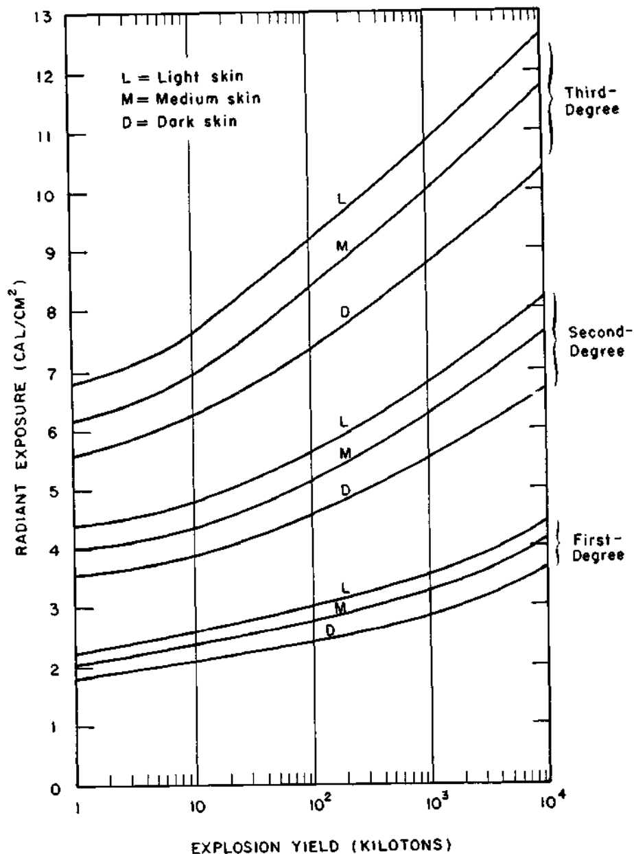
Figure 12.64. Radiant exposure required to produce skin burns for different skin pigmentation levels.
