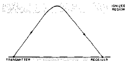
Figure 10.08. Reflection of a radio (or radar) wave by successive refractions in an ionized region of the atmosphere.
