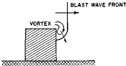
Figure 4.27. Blast wave moving down rear of cube.
