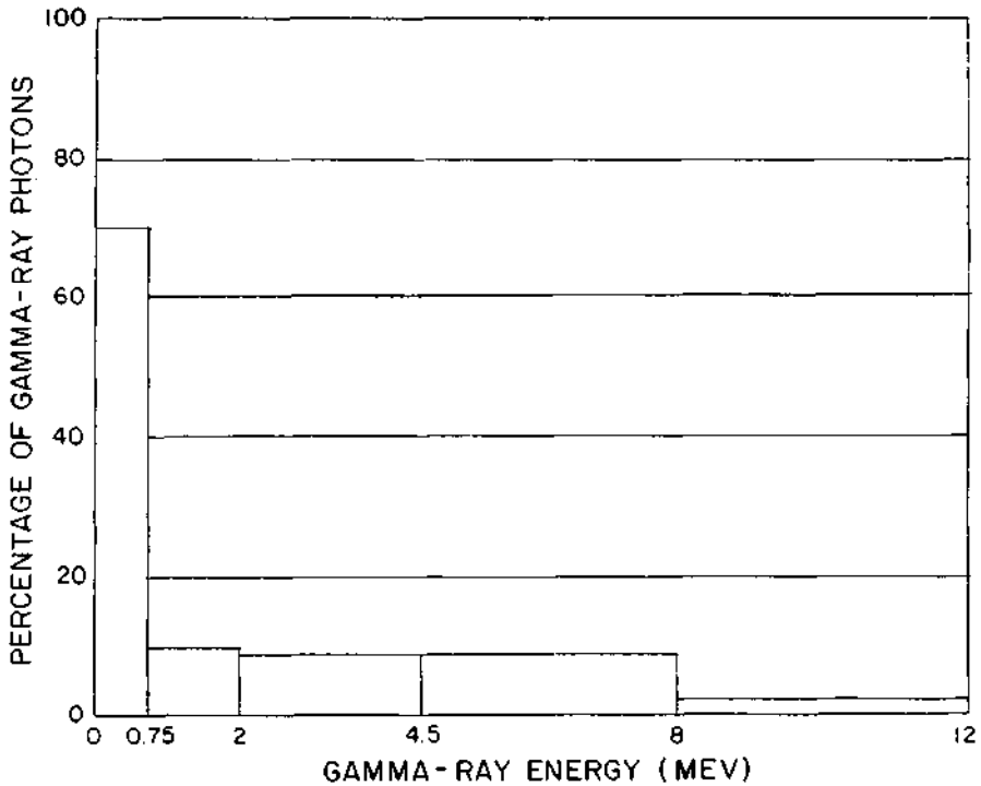
Figure 8.106. Spectrum of initial gamma radiation 2,000 yards from a 20-kiloton explosion.
