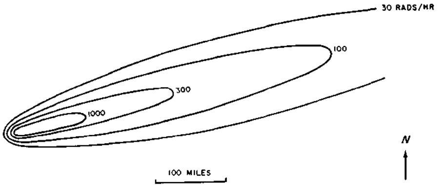
Figure 9.100a. Idealized unit-time reference dose-rate contours for a 10-megaton, 50-percent fission, surface burst (30 mph effective wind speed).
