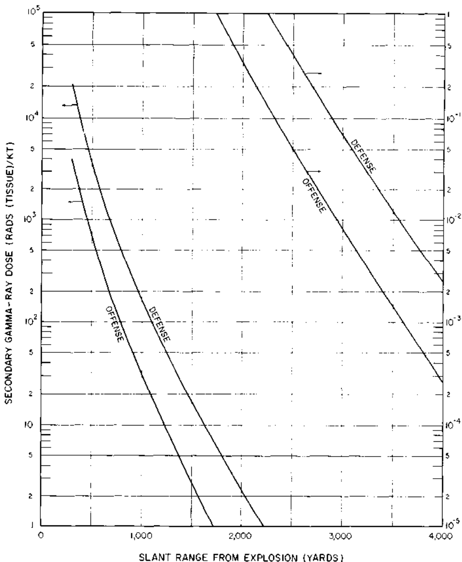
Figure 8.127a. Air-secondary gamma-ray component of the initial nuclear radiation dose per kiloton yield as a function of slant range from fission weapon air bursts, based on 0.9 normal sea-level air density.
