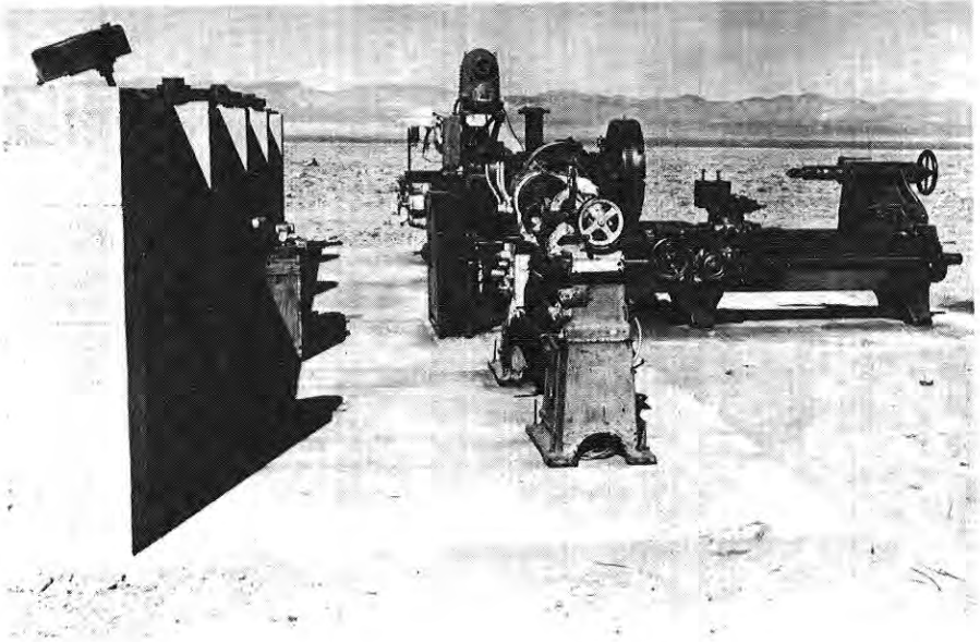
Figure 5.128. Machine tools behind masonry wall before a nuclear explosion, Nevada Test Site.
