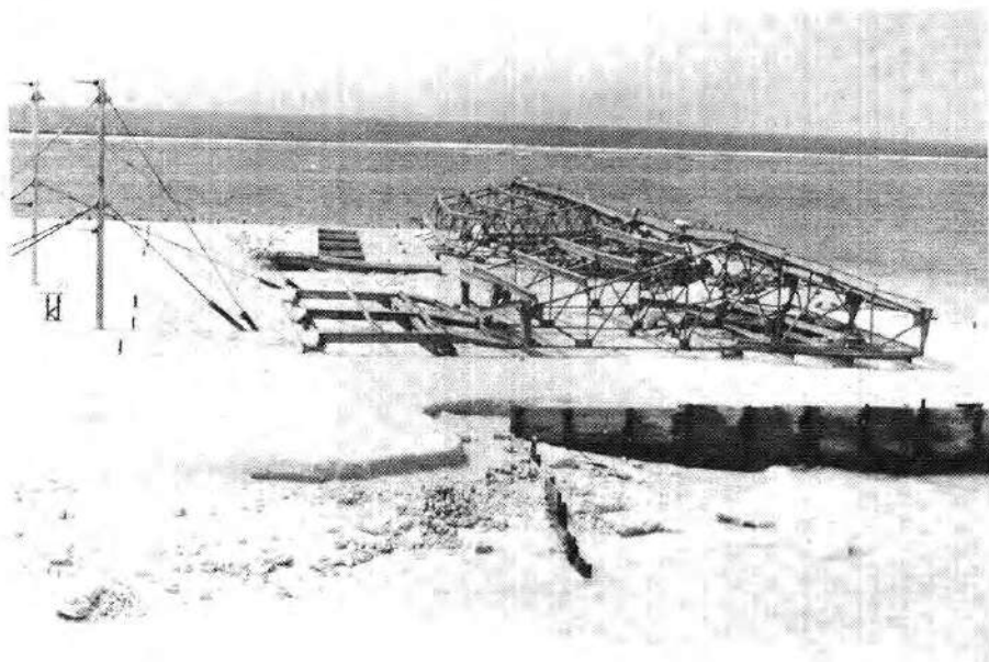
Figure 5.51a. Structure similar to Figure 5.48a after exposure to 6.1 psi peak overpressure and 0.6 psi dynamic pressure; positive phase duration several seconds.
