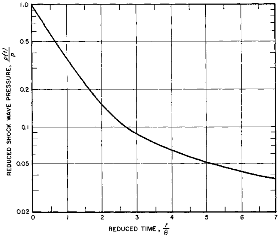
Figure 6.116b. Pressure-time relationship for water shock waves from nuclear explosion in deep isovelocity water; p is the peak pressure and p(t) is the value at time t after arrival of the shock front.
