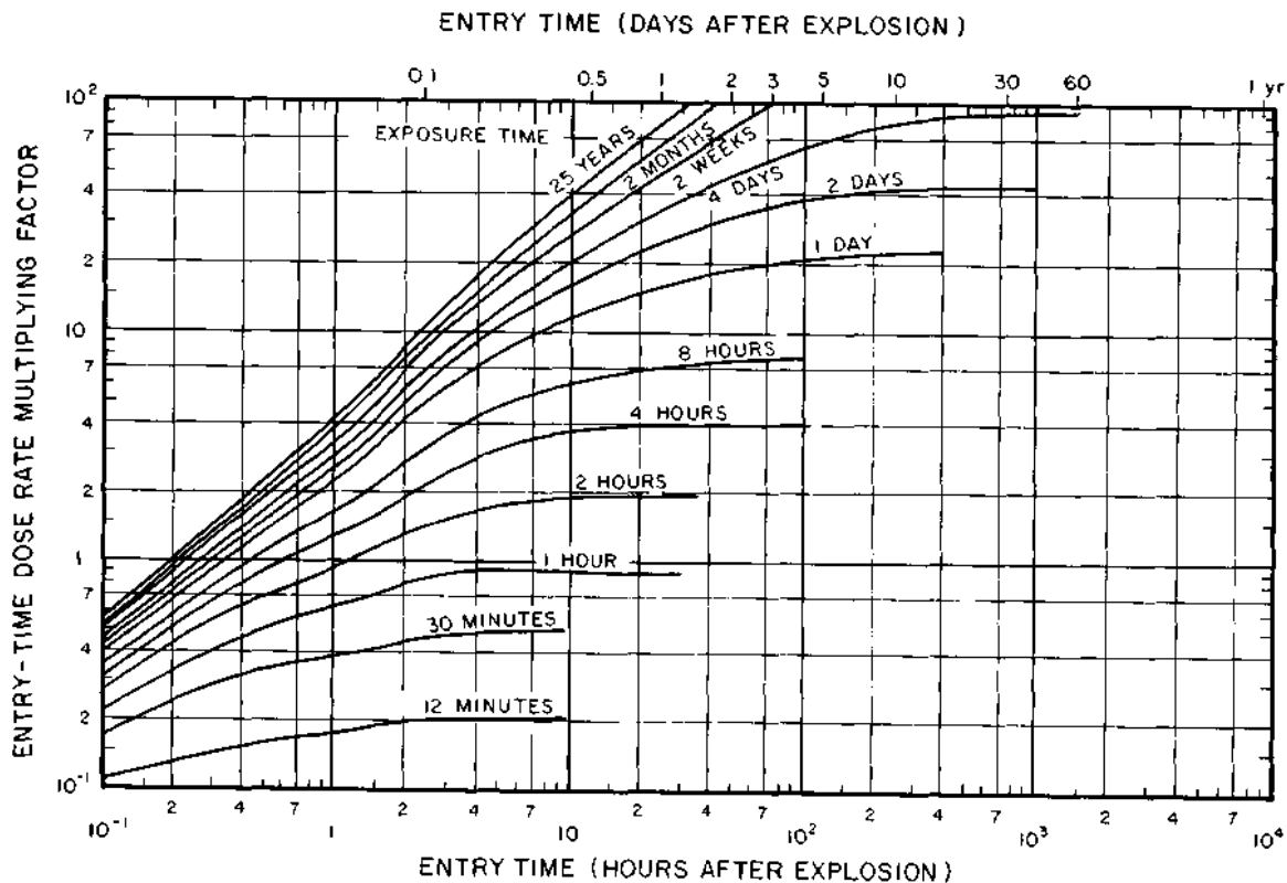
Figure 9.27. Curves for calculating accumulated radiation dose from early fallout based on dose rate at time of entry.
