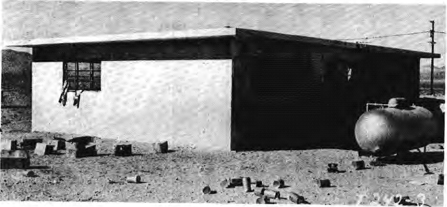
Figure 5.73. Reinforced precast concrete house after a nuclear explosion (5 psi peak overpressure). The LP-gas tank, sheltered by the house, is essentially undamaged.
