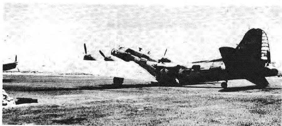
Figure 5.95a. Aircraft after side exposed to a nuclear explosion (3.6 psi peak overpressure).
