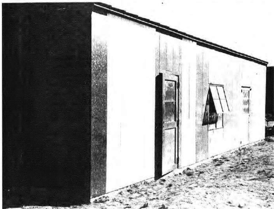
Figure 5.40a. Exterior of self-framing steel panel building before a nuclear explosion, Nevada Test Site.
