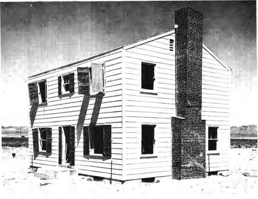
Figure 5.65. Strengthened wood-frame house after a nuclear explosion (2.6 psi peak overpressure).
