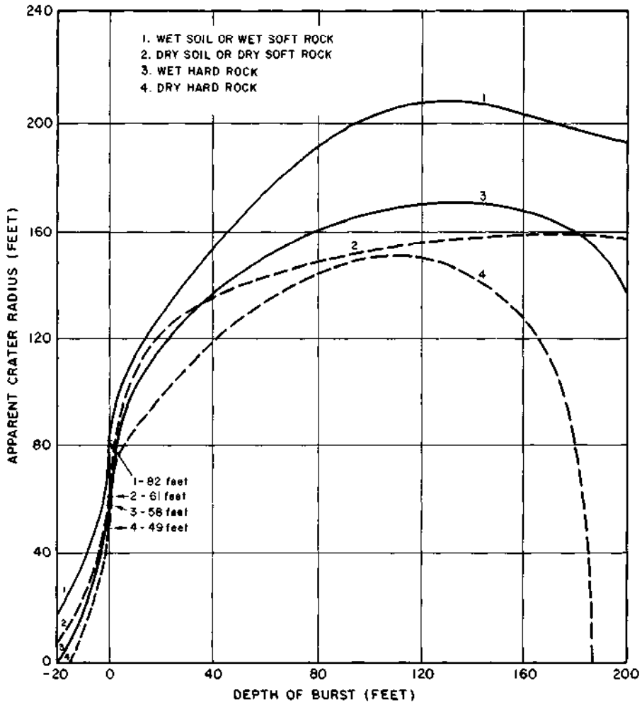
Figure 6.72a. Apparent crater radius as a function of depth of burst for a 1-kiloton explosion in (or above) various media.
