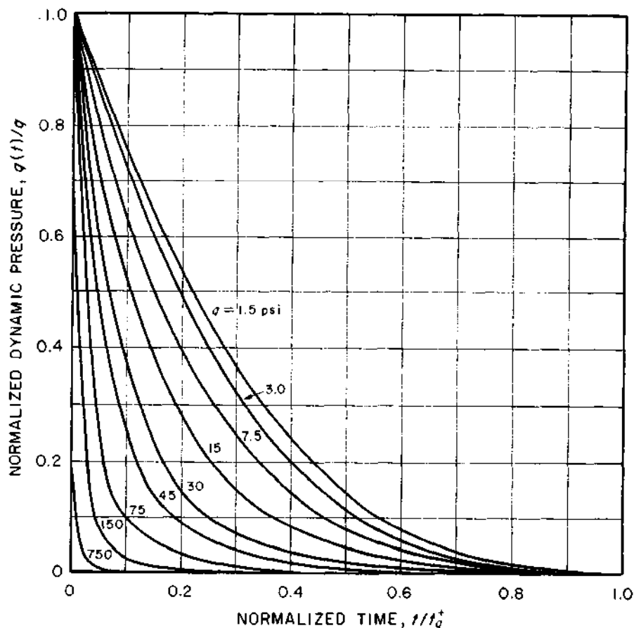
Fig. 3.58. Rate of decay of dynamic pressure with time for several values of the dynamic pressure.
