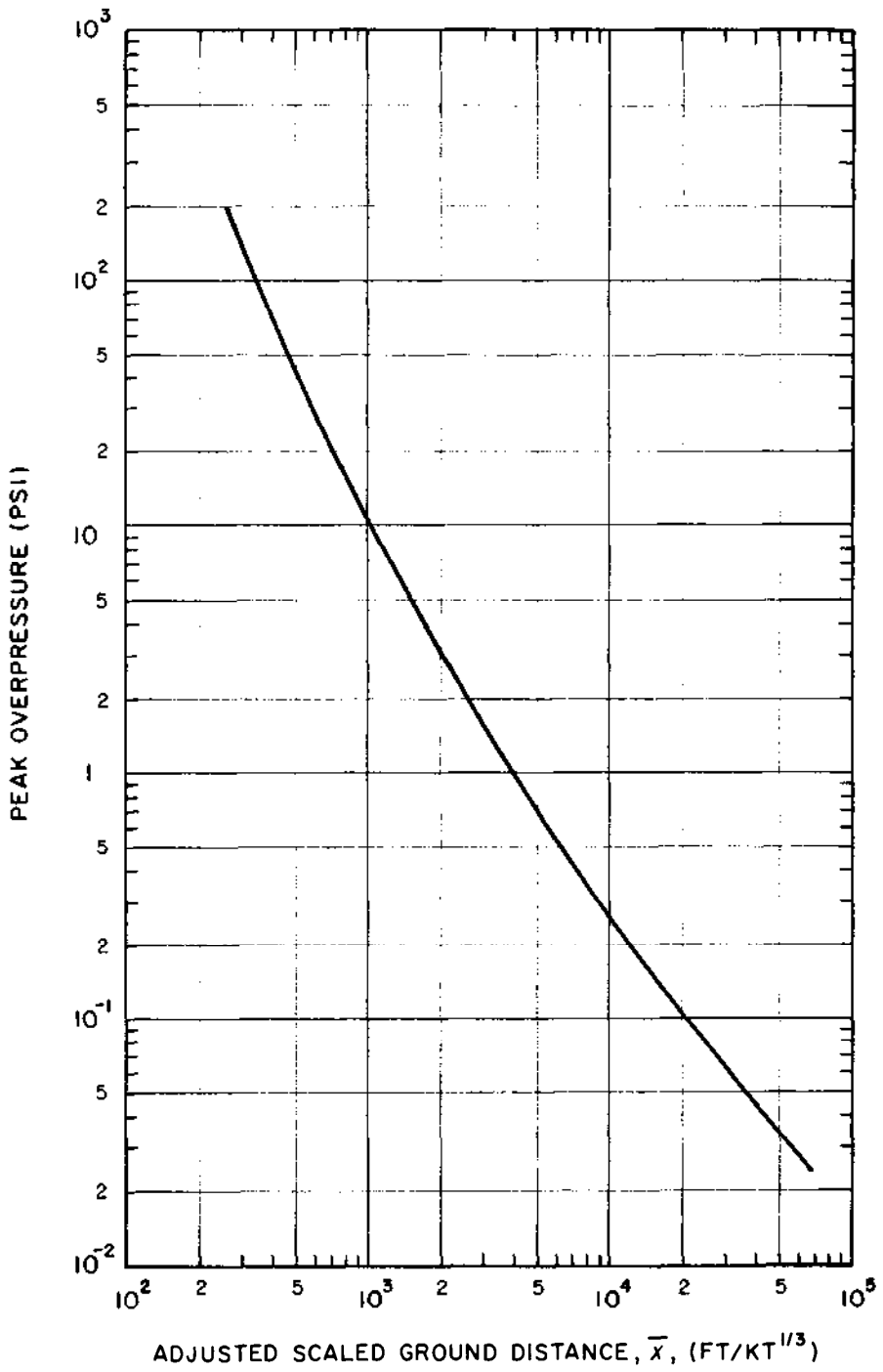
Figure 6.81. Peak overpressure of air blast from an underground explosion as a function of adjusted scaled ground distance from a buried 1-kiloton explosion.
