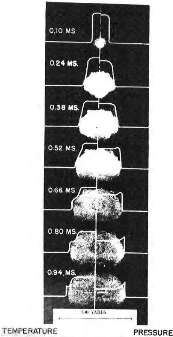
Figure 2.118. Variation of temperature and pressure in the fireball. (Times and dimensions apply to a 20-kiloton air burst.)
