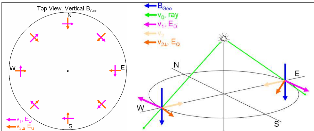
Figure 4-14. Including the quadrupole term in the simple case. This is for the same case as in Figure 4-13, but with the quadrupole term now added. This term (in orange) is radial, and also has cylindrical symmetry. The vectors in the right drawing shows the quadrupole term (dark orange) is from only part of the second turning electron motion (lighter orange) – only the transverse part of the field generated from v_2 can propagate outward along the ray. Thus, we decompose the light orange vector into a part along the green ray line (not shown) and the part that is perpendicular (dark orange – it has a vertical and radial part).
