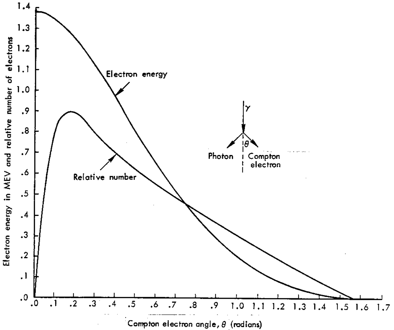
Fig. 3 — Energy and number distribution for Compton scattering: 1.6-MEV \gamma
