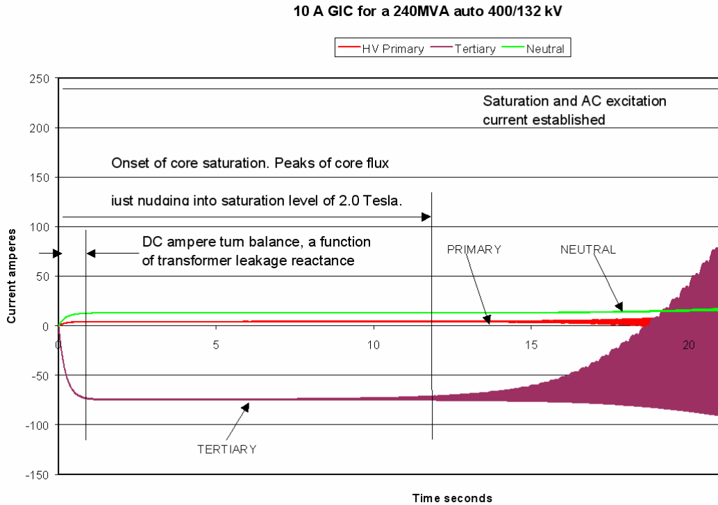
Figure A2-11. Analysis of saturation delay for 240MVA 400/132kV auto transformer with 10 Amperes of step DC input.
