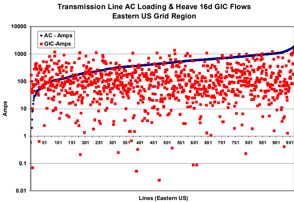
Figure 4-24. Summary of combined Eastern U.S. Grid transmission line simultaneous AC and GIC current loadings for Heave Case 16d.
