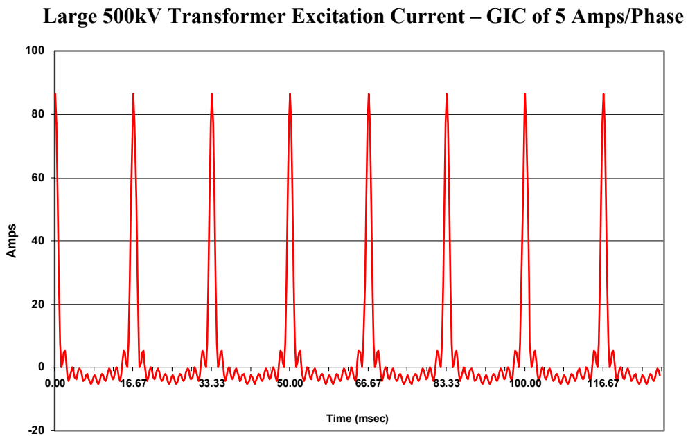
Figure 2-41. Distorted excitation Current with 5 Amps/phase of GIC.
