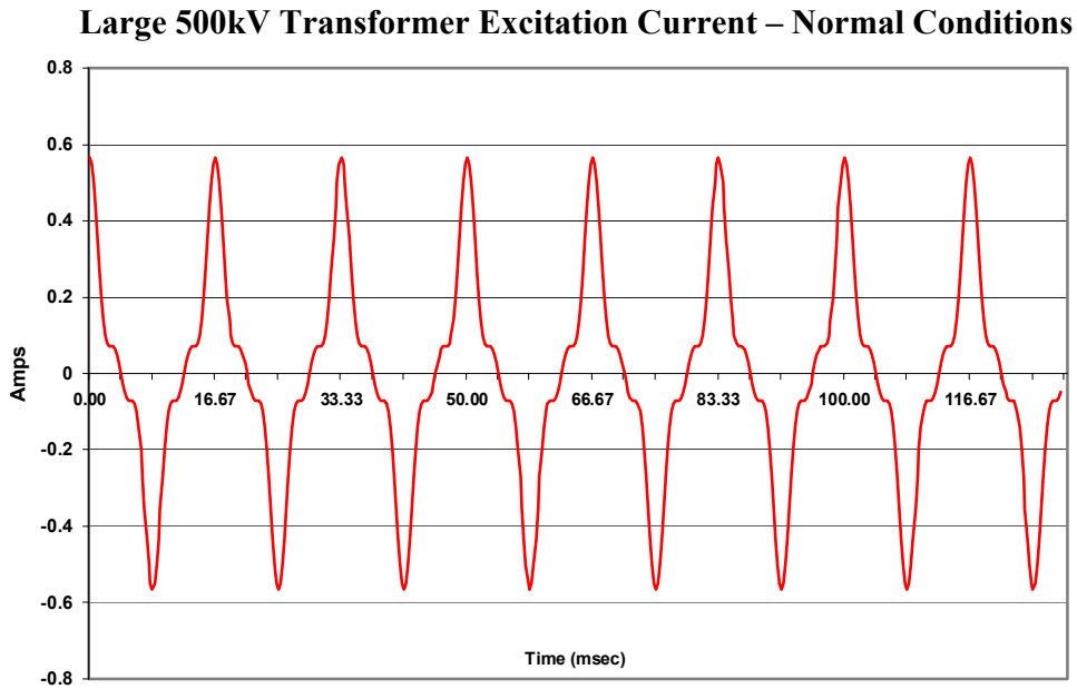
Figure 2-40. Normal excitation current in 500kV transformer.
