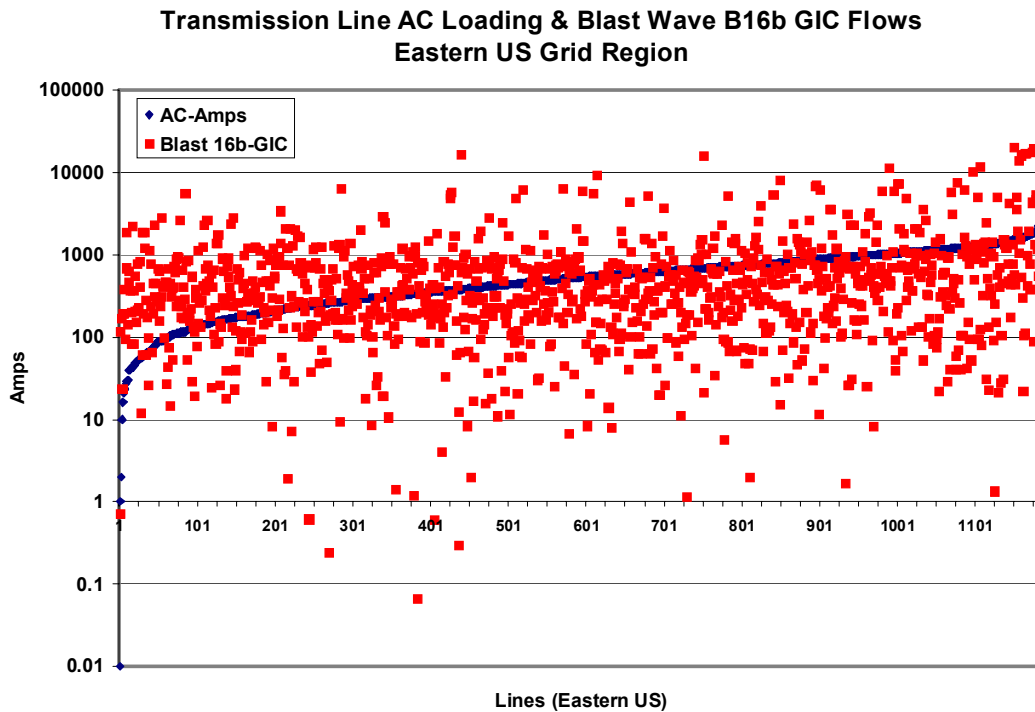
Figure 4-12. Summary of combined Eastern U.S. transmission line simultaneous AC and GIC current loadings for Case B16b, using SERC powerflow model.
