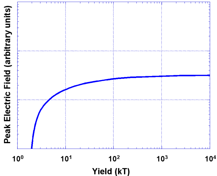
Figure 2-13. Yield scaling for peak E3B electric field.
