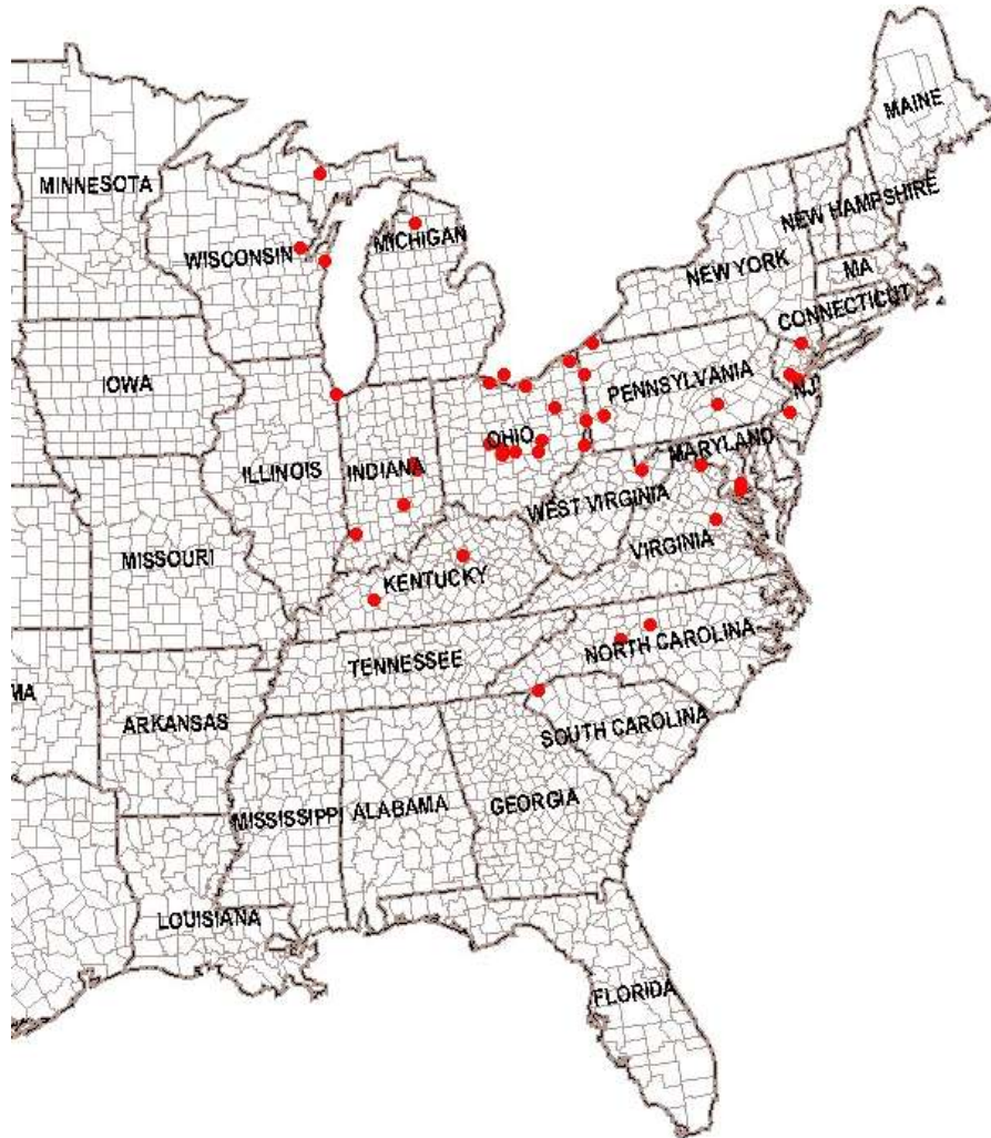
Figure 5-23. Case 16d region - location of transformers at risk, GIC of 200 Amps or greater per phase.
