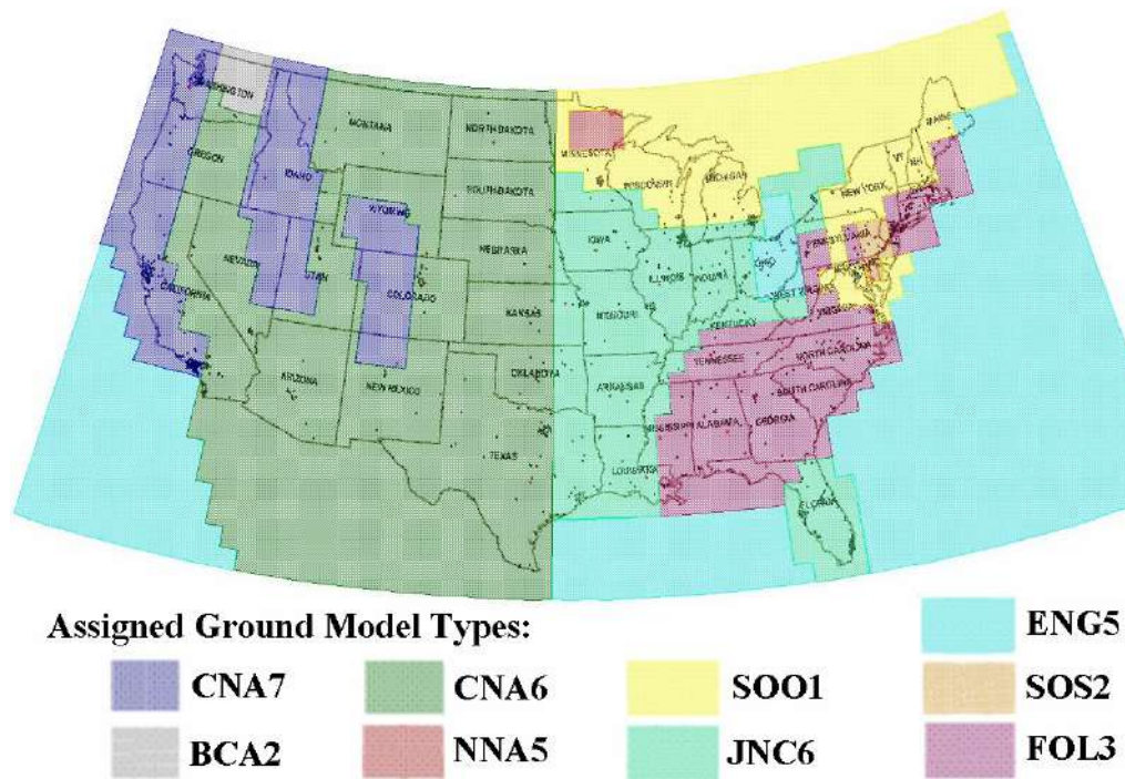
Figure 2-22. Multiple 1-D ground models for the U.S. grid.
