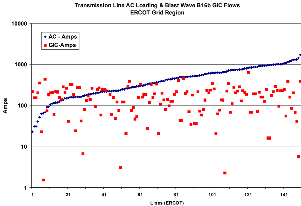
Figure 4-15. Summary of combined ERCOT transmission line simultaneous AC and GIC current loadings for Case B16b.
