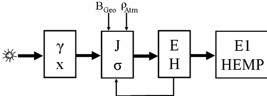
Figure 4-8. Overview of E1 HEMP generation theory terms. Gammas (and x rays, of less importance) interact with the air (with its variation of density, \rho_{\text{Atm}} , with altitude), producing source current (from the geomagnetic field, B_{\text{Geo}} , turning the Compton electrons) and conductivity. The current generates the electromagnetic field (E and H), as moderated by the conductivity. The EM field propagates away as the E1 HEMP.
