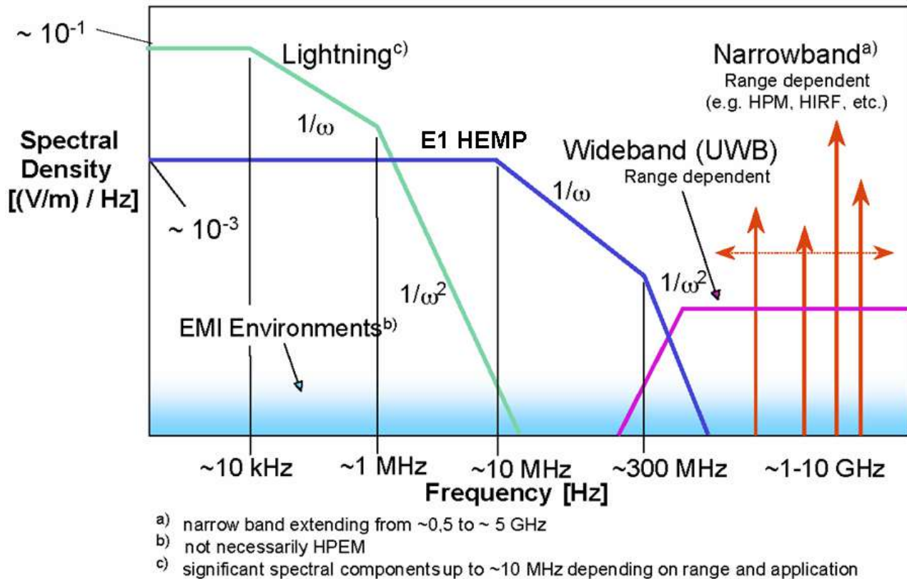
Figure 2-5. Approximate EM spectrums for various EM disturbances. E1 HEMP dominates in the range of about 1 MHz to several hundred MHz. IEMI is represented by the “Wideband” and “Narrowband” signals on the upper frequency (right) side.
