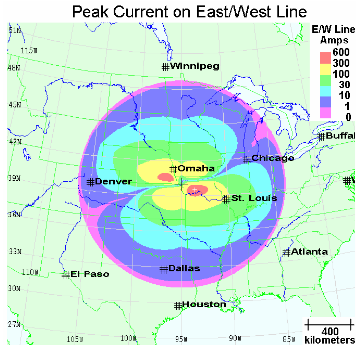
Figure 2-31. Sample contour plot of the peak current on an east/west line. This is the same as in the previous figure, but with the line going east and west. (Parameters: 10^{-3} S/m ground conductivity, line 5 meters off ground, line 100 meters long, wire 0.2 centimeters in radius.)
