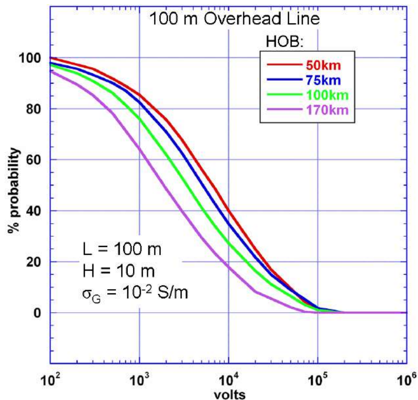
Figure 7-1. Voltage distribution for a 100-meter long horizontal power line. The results are for a typical burst, for four burst heights over the U.S. The power line is 10 meters over 10^{-2} \text{ S/m} ground.
