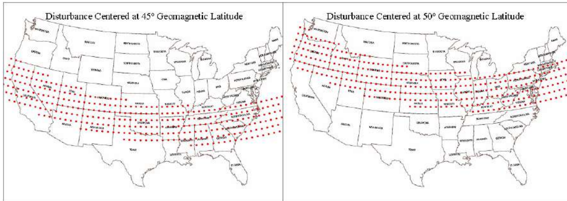
Figure 3-22. Disturbance regions for 45° and 50° geomagnetic latitude storms.
