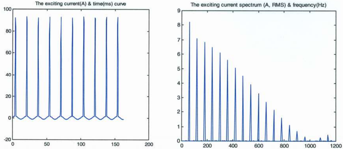
Figure A4-5. The exciting current waveform and frequency spectrum calculated for a GIC of 75 amps in neutral (230/115 kV, 3-legged, 3-phase core form auto-transformer).
