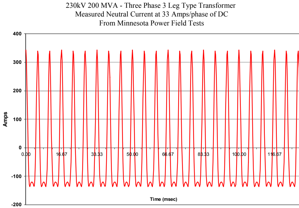
Figure A4-15. Measured neutral current for 3-phase, 3-legged core form transformer with GIC present.
