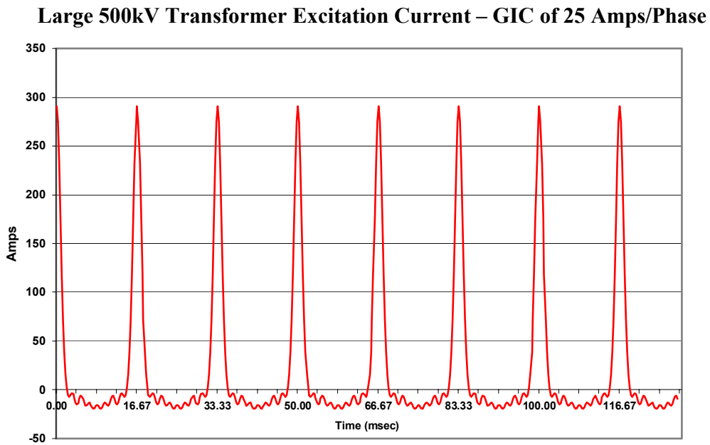
Figure 1-26. Distorted excitation current with 25 amps/phase of GIC.
