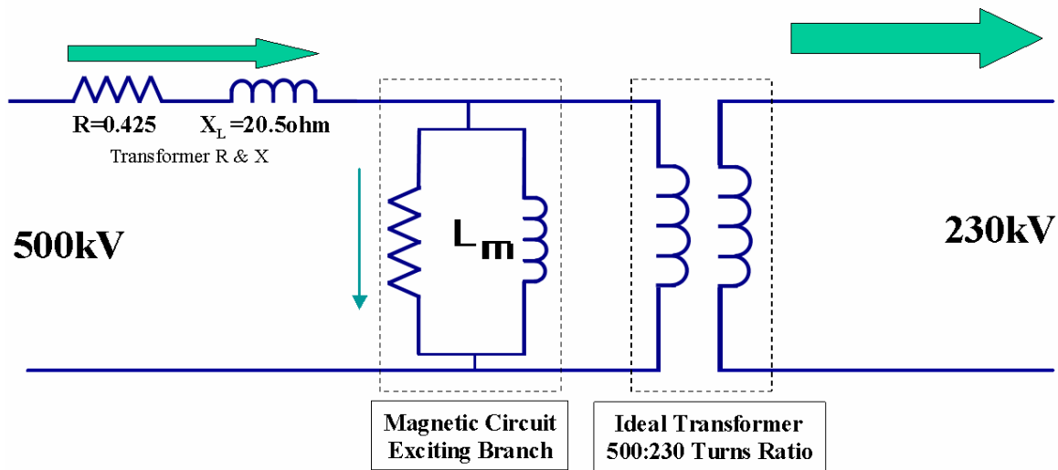
Figure A4-24. Simple equivalent one-line diagram of 500/230kV transformer model.
