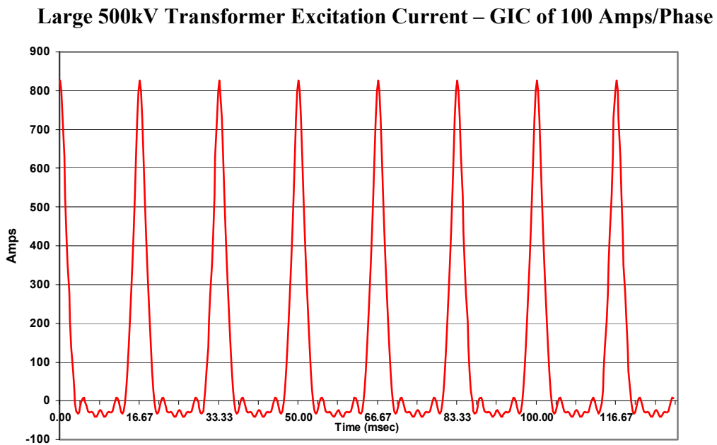
Figure 1-27. Distorted excitation current with 100 amps/phase of GIC.
