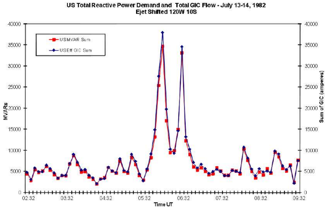
Figure 3-21. GIC and MVAR demand variations for the U.S. power grid during the July 13-14, 1982 geomagnetic storm with 120° longitude and 10° latitude shift.
