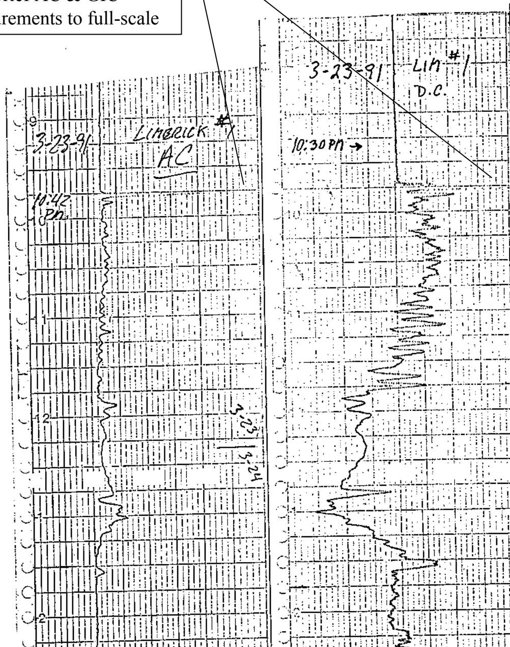
Figure A3-21. Observed GIC and neutral AC current at Limerick on March 24, 1991 (times above are EST, not UT).
