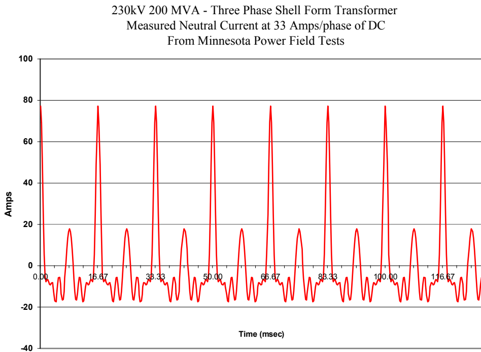
Figure A4-16. Measured neutral current for 3-phase shell form transformer with GIC present.
