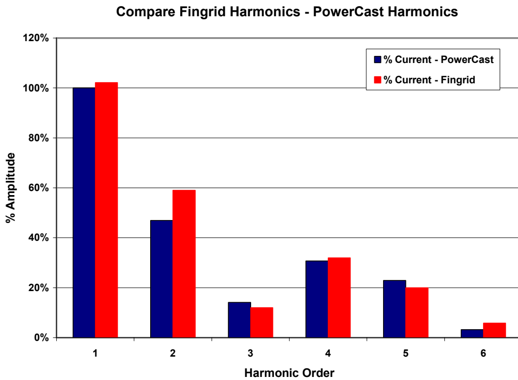
Figure A4-10c. Comparison of observed and calculated AC harmonics for 5-legged core form transformer.
