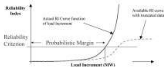
Figure 4-3 Reliability Curve Plotted Against Load Increases
