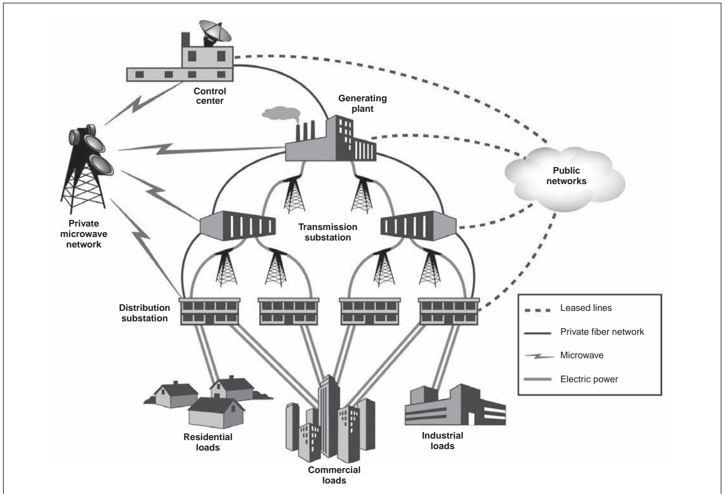
Figure 2: Overview of the Electric Power System and Control Communications
