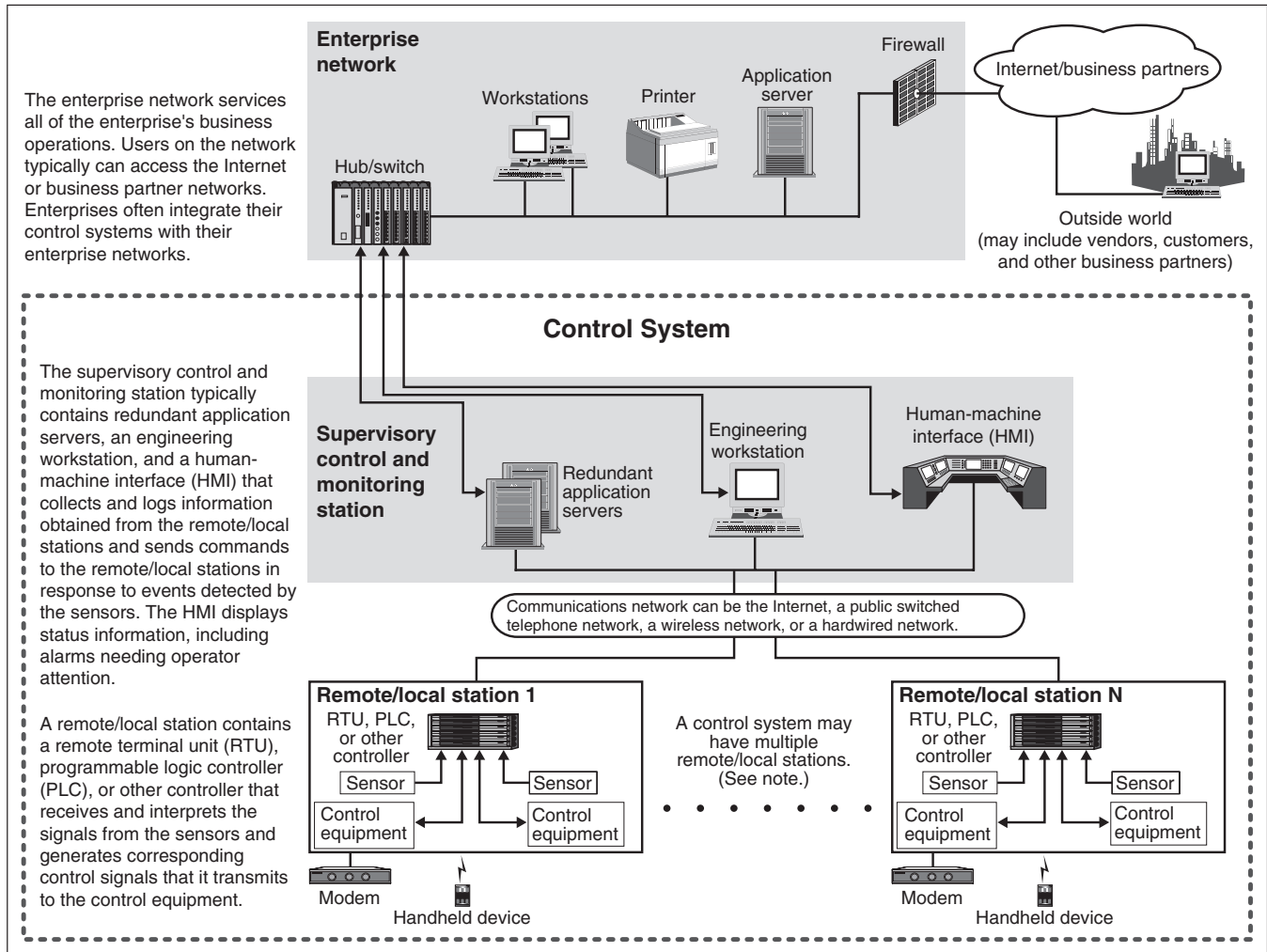
Figure 3: Typical Components of a Control System
