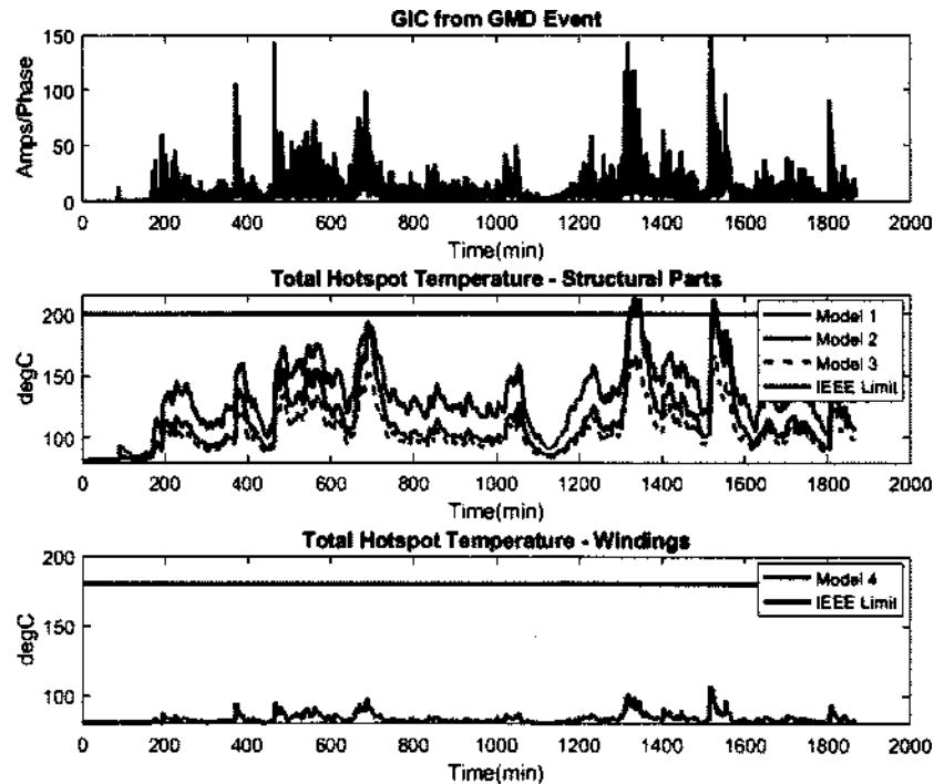
Figure 2 Simulation of transformer hotspot temperatures using a GIC waveform representative of the March 1989 GMD Event
