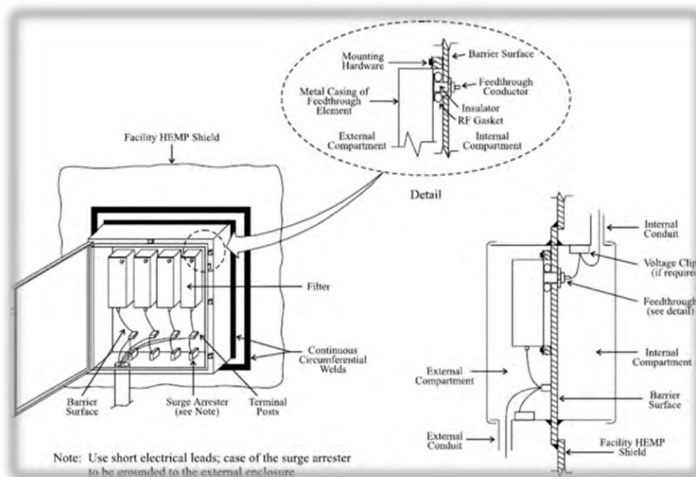
Figure 6. Typical cable POE protection design
