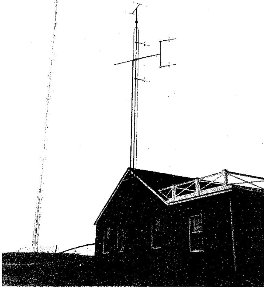
AM BROADCAST STATION ANTENNA AND TRANSMITTER BUILDING
