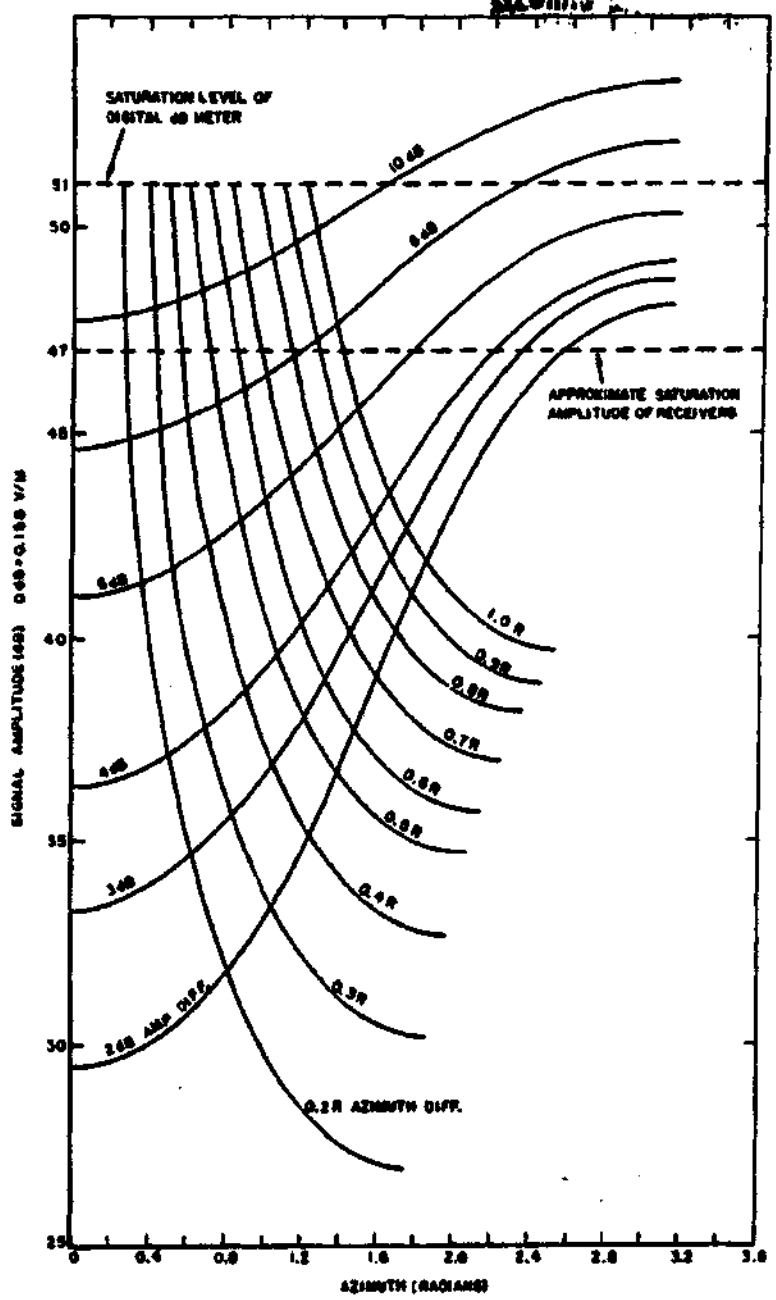
FIGURE 4. RECEIVED SIGNAL FROM A 500 W/M AT 1 km SOURCE AT STATION OBSERVING THE LARGER AMPLITUDE VALUE.
