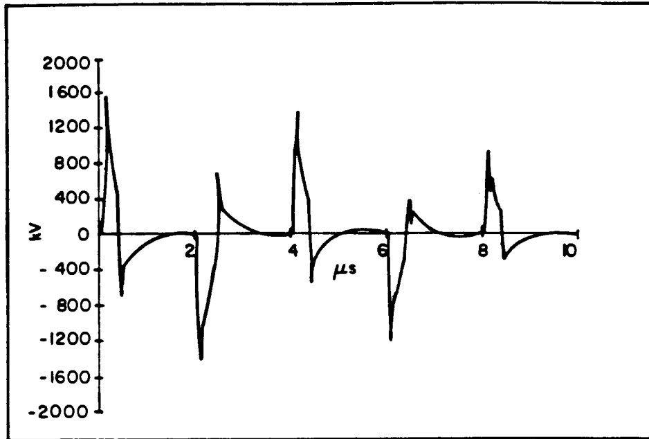
a) Towers spaced at 300m from each other, V_{fo}=500 kV.
