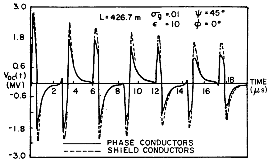
a) Phase conductor and shield conductor voltages for shield wires ungrounded at z=L
