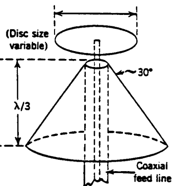
(f) Discone antenna
