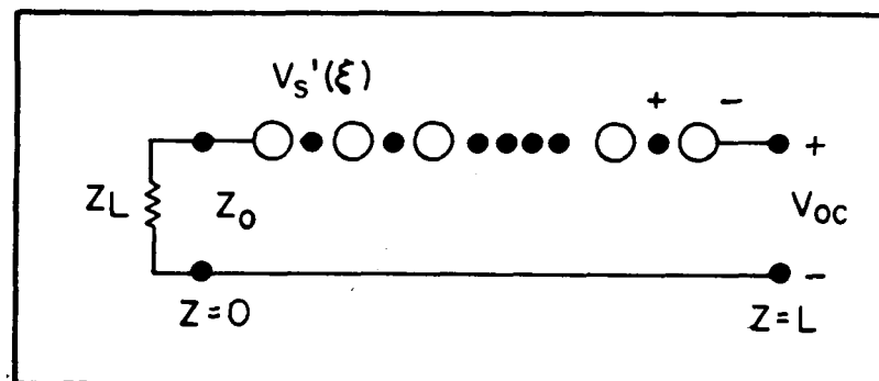
Fig. 16b. Distributed source excitation.
