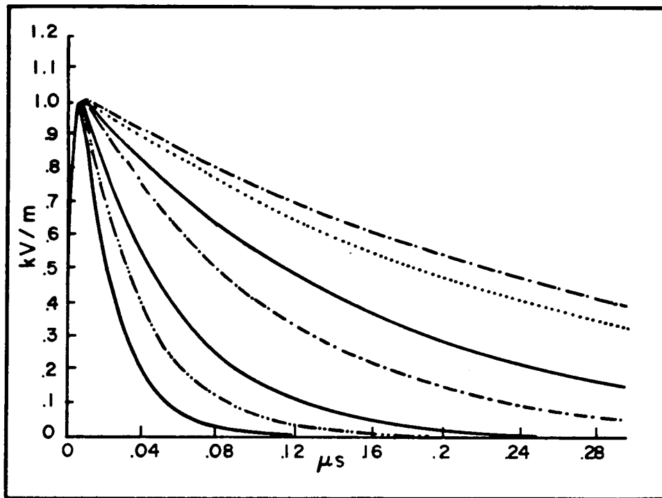
Fig. B4a. Normalized waveshapes of incident electric fields waveshapes.
