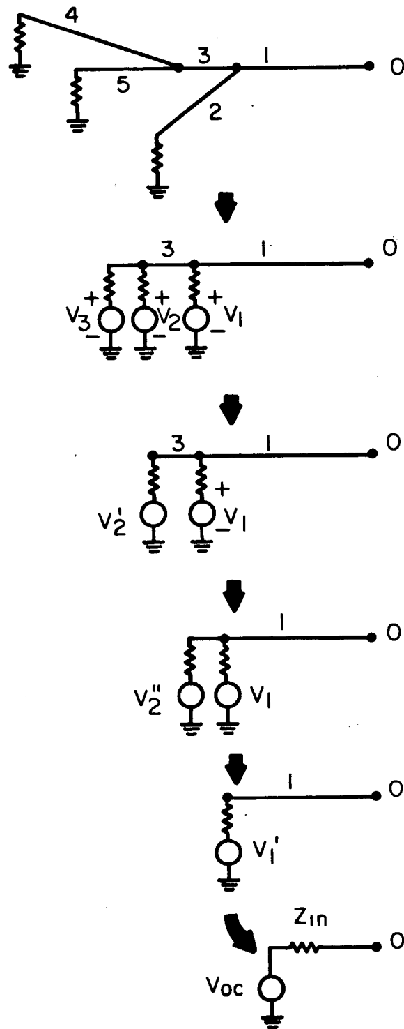
Fig. 25. Series of transformations of network to a Thevenin equivalent.
