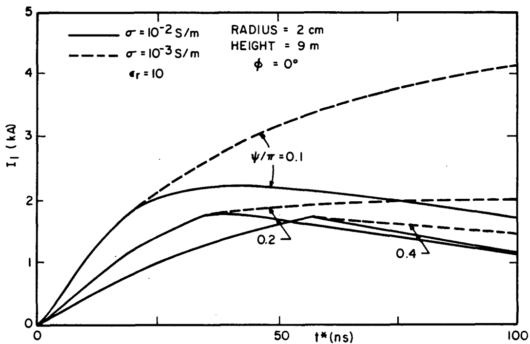
Fig. C8. Total current induced on conductor #1 which is 9 m away from conductor #2 and at the same height as #2 from ground for conductivity \sigma = 10^{-2} S/m or \sigma = 10^{-3} S/m. At "+", a multiple scattered field will arrive at wire #1 [C5].
