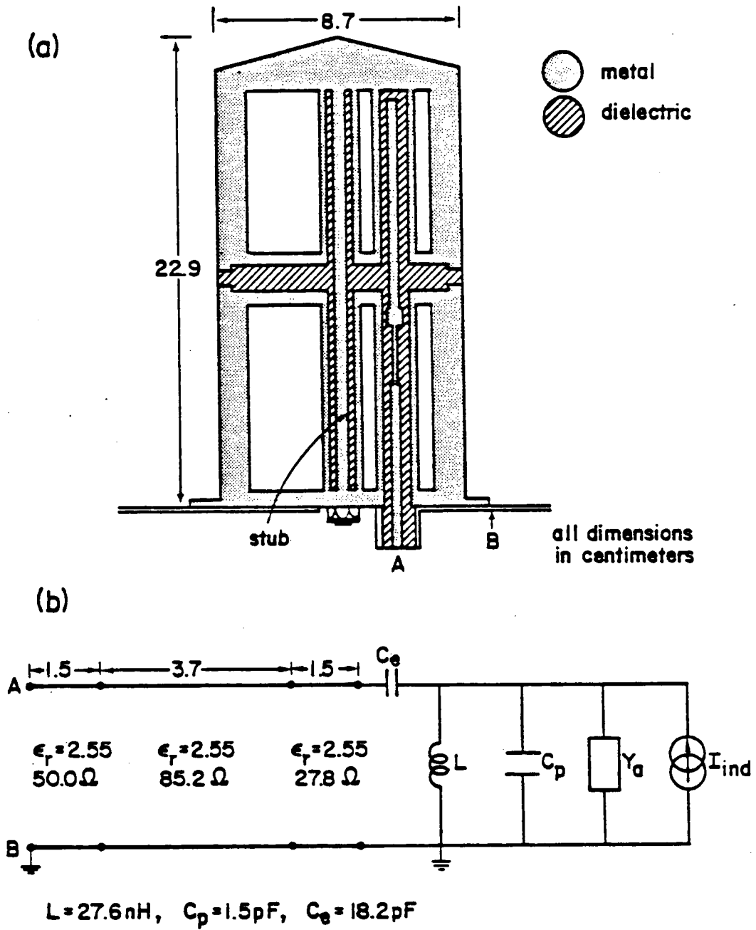
Fig. 44. Schematic diagram and equivalent circuit of the UHF Communication Antenna.
