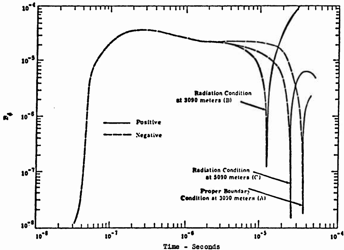
Figure 17. B_\phi at 2000 Meter Range.
